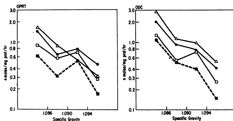
FIGURE 5 Orotate phosphoribosyltransferase (OPRT) and orotidyl de-carboxylase (ODC) in circulating erythrocytes of different density after initiation of therapy with oxipurinol (800 mg/day) in patient W. H. H. Mean activity is plotted against specific gravity (increasing values correspond to increasing cell age in vivo). Control, ■ --- ■; allopurinol therapy (solid lines); day 3, □ — □; day 10, ● — ●; day 13 and 17, △ — △.
