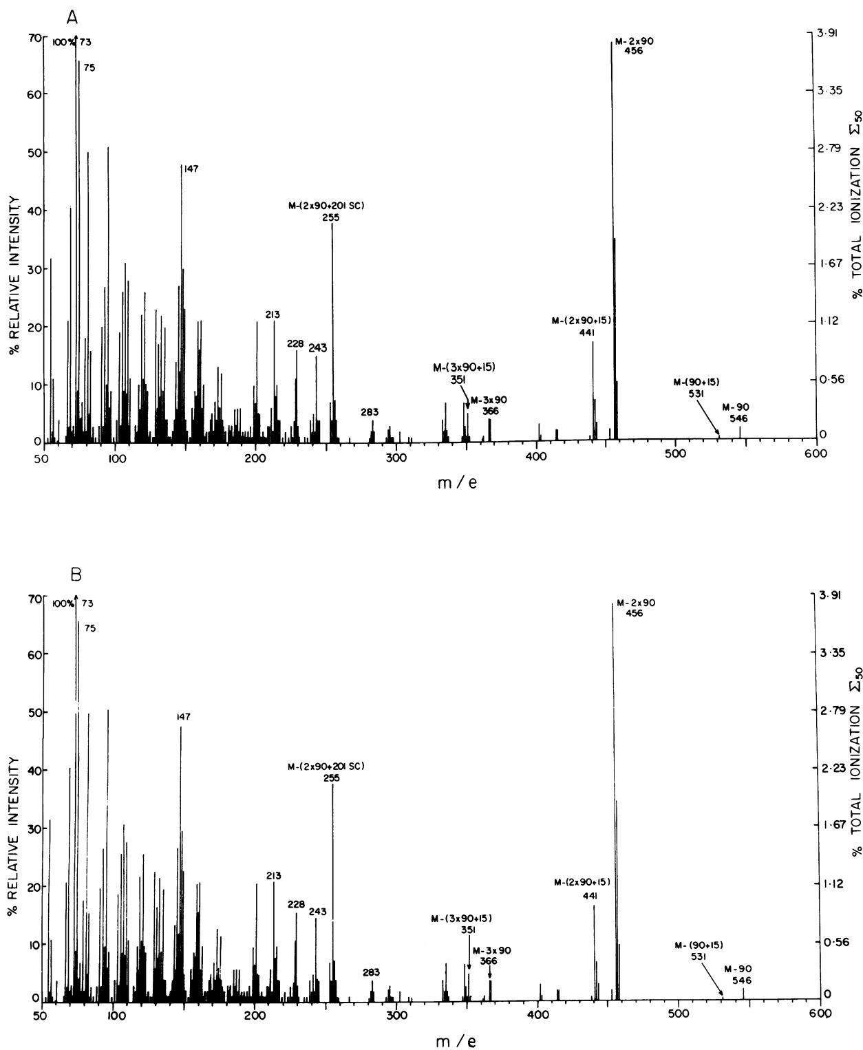
FIGURE 2 Mass spectrum of the biosynthetic 5β-cholestane-3α,7α,26-triol (25R) obtained from a large scale incubation experiment with human liver mitochondria (A) compared with the authentic compound (B).
