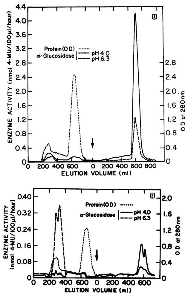
FIGURE 4 Chromatography on a Sephadex G-100 column of crude lysate supernatant fluids from cultured skin fibroblasts. Fractions of 10 ml were collected. The arrow indicates addition of maltose to the eluant. 4-Methylumbelliferyl- \alpha -D-glucopyranoside was used as substrate. 4-MU = 4-methylumbelliferone. (A) Normal fibroblasts. (B) Adult acid \alpha -glucosidase deficiency fibroblasts.
