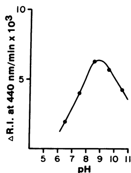
Figure 6. Effect of pH on elastin-separated platelet lysate elastase-like activity. The sample was added to compound I in 0.04 M Tris HCl, pH 7.5—10% dimethylsulfoxide (see Methods), and different pH values were obtained by addition of small quantities of concentrated HCl or NaOH. R.I., relative intensity.
