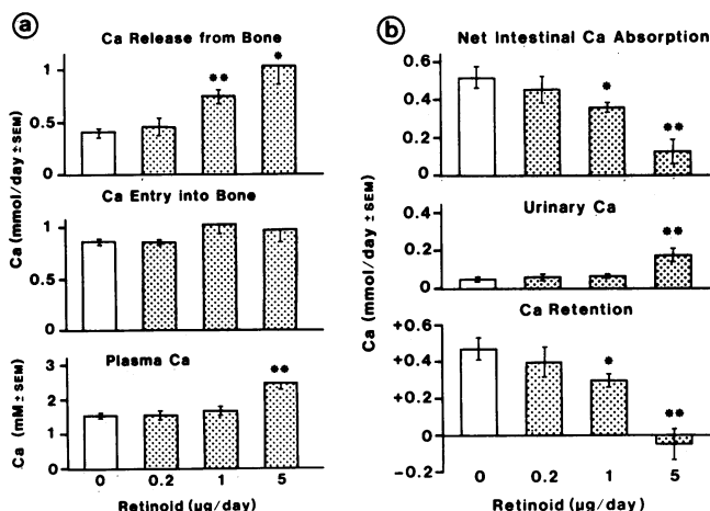
Figure 2. Effect of retinoid on Ca balance and ^{45}\text{Ca} kinetics in TPTX rats. Animals were treated with retinoid for 9 d, and Ca balance and ^{45}\text{Ca} kinetics were performed during the last 3 d of treatment, as described in Methods. Values are means \pm SEM of four animals (0 and 1 \mu\text{g} ) or three animals (0.2 and 5 \mu\text{g} ) per group. * P < 0.05; ** P < 0.01, as compared with controls by Student's two-sided t test.
