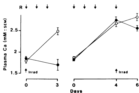
Figure 8. Effect of irradiation on retinoid-induced hypercalcemia in TPTX rats. All animals were given retinoid (R) at 25\text{ }\mu\text{g/rat} . Values are means \pm SEM, n = 4-5 . (○) Retinoid; (●) retinoid and irradiation at time points indicated by arrows.
