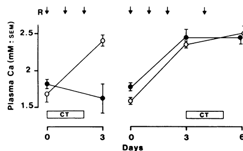
Figure 9. Effect of calcitonin (CT) on retinoid-induced hypercalcemia in TPTX rats. All animals were given retinoid (R) at 25\text{ }\mu\text{g/rat} . 8 IU/kg per d CT was given for 3 d as indicated. Values are means \pm SEM, n = 4-5 . (○) Retinoid; (●) retinoid + CT.
