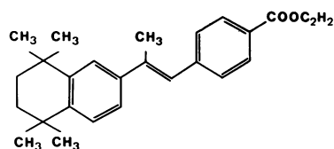
Chemical structure of the retinoid Ro 13-6298.
