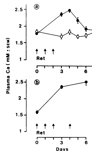
Figure 4. Effect of retinoid on plasma Ca in TPTX rats. Animals were given solvent (○) or 25 \mu g of retinoid (●) on days 0, 1, and 2 (a), or on days 0, 1, 2, and 4 (b). Values are means \pm SEM. No. of animals was 4 in the solvent group (a) and 5 in all other groups.
