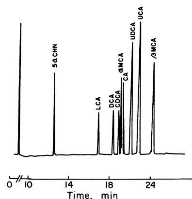
Figure 1. Capillary gas liquid chromatogram of trimethylsilyl ether methyl ester derivatives of bile acids. The bile-acid derivatives were separated by capillary GLC. 5 \alpha -Cholestane (5 \alpha -CHN) and UDCA were the internal and recovery standards, respectively. The derivatized bile acids separated were: LCA, lithocholic acid; DCA, deoxycholic acid; CDCA, chenodeoxycholic acid; \alpha -MCA, \alpha -muricholic acid; CA, cholic acid; UCA, ursodeoxycholic acid; and \beta -MCA, \beta -muricholic acid.
