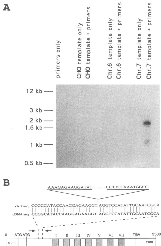
Figure 8. PCR amplification of the human CTR gene from human-hamster somatic cell hybrids. Human-hamster somatic cell hybrid DNA that contained either human chromosome 6 or chromosome 7 was chosen to verify the chromosome 7 location of the CTR gene indicated by the in situ hybridization results (see Results and Fig. 7). Primers derived from human CTR sequences corresponding to two exons identified in the mouse CTR gene were used. (A) Southern blot of PCR reaction products using an o-hCTR cDNA probe. This blot demonstrates that the human CTR primers are specific for human DNA from the hybrid containing chromosome 7 and not chromosome 6. The ~2-kb PCR product obtained is consistent with the presence of an intron between the two exon based primers. (B) Diagram showing partial sequence obtained from the ~2-kb PCR product amplified from the chromosome 7 containing hybrid. The location of the PCR primers in the o-hCTR cDNA is indicated by arrows. The PCR product sequence shown (designated ch. 7 seq. ) includes parts of two exons interrupted by intron sequence (inserted at top). Taken together, the data shown in Figs. 7 and 8 demonstrate that the CTR gene is located on chromosome 7 at band q22.
