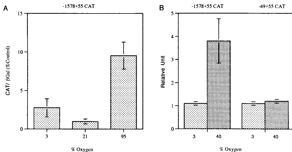
Figure 4. Hyperoxia activates \gamma GT- P_{III} -CAT in SV40T-T2 and HepG2 cells. Cells were transfected with DNA, exposed to various oxygen concentrations, then extracted as described in Methods. CAT activity was normalized by \beta -galactosidase activity to correct for transfection efficiency. A shows \gamma GT (-1578+55)-CAT in SV40T-T2 cells in 3, 21, or 95% oxygen. B shows the same construct plus \gamma GT(-49+55)-CAT in HepG2 cells in 40% oxygen relative to that in 3% oxygen.
