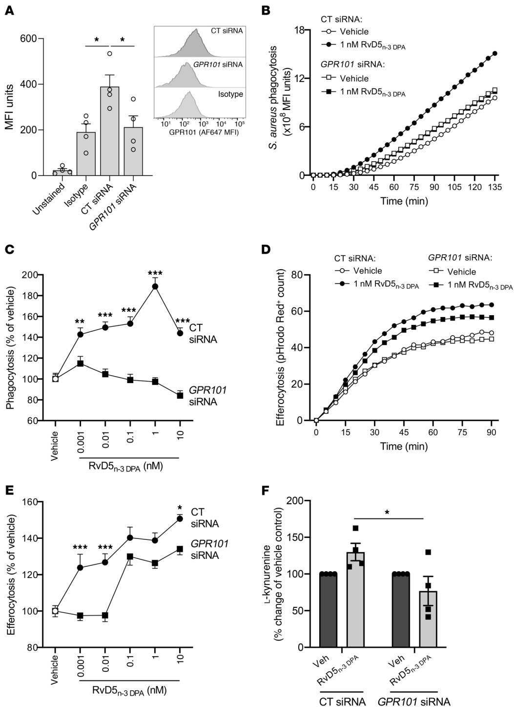
Figure 5. GPR101 mediates the protective actions of RvD5 n-3 DPA on human macrophages. (A)
